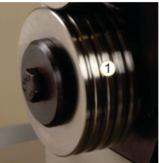
1 ALRX6520B-02-02 : Roller (Garedi) with Special Groove
